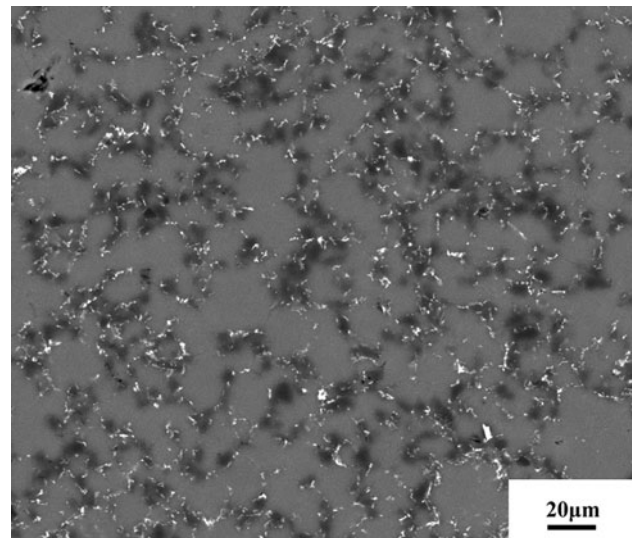
Fig. 6 SEM micrograph of sample 5
