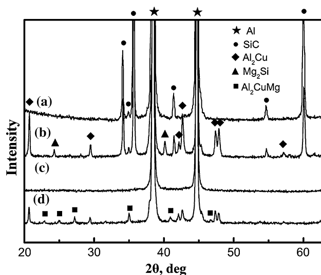
Fig. 10 XRD patterns of (a) sample 6 after solution treatment, (b) sample 6, (c) sample 7 after solution treatment, and (d) sample 7
