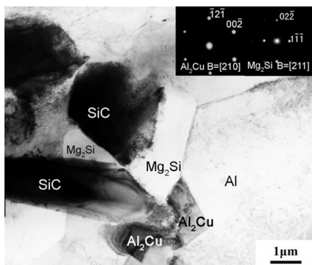
Fig. 8 TEM micrograph of sample 6
