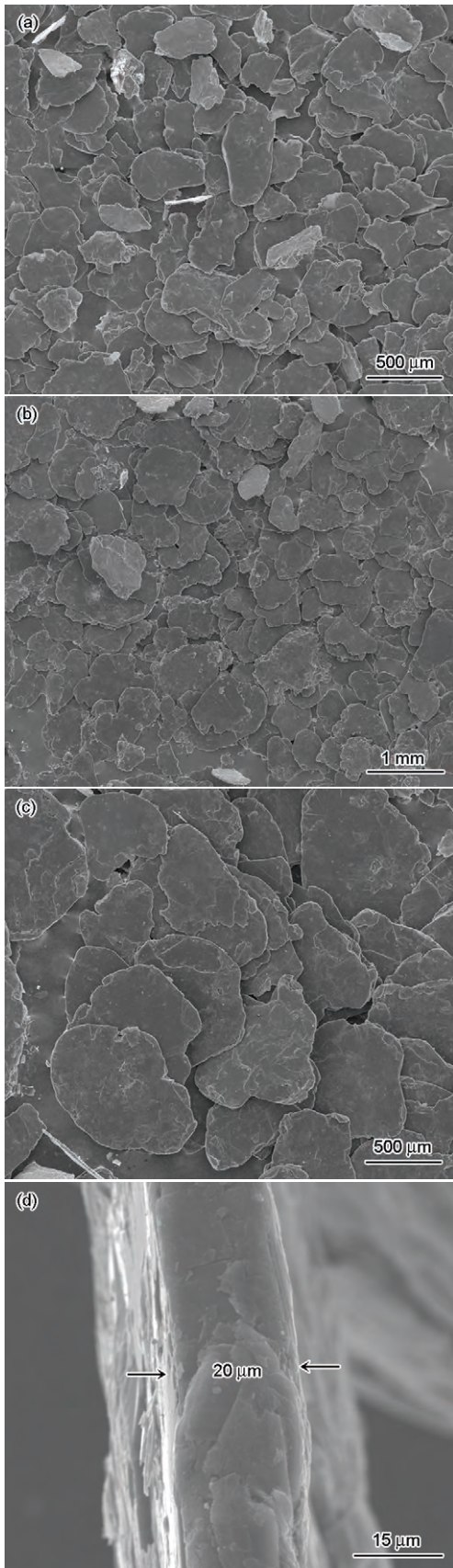
图1 不同尺寸片层石墨的SEM像 Fig.1 SEM images of graphite flakes in different sizes (a) 150 μm (b) 300 μm (c) 500 μm (d) side of the 500 μm graphite flake
