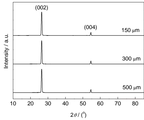
图2 不同尺寸片层石墨的XRD谱 Fig.2 XRD spectra of graphite flakes in different sizes
