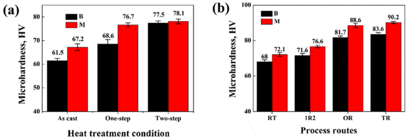
Fig. 7 – Microhardness of B and M alloys with different: (a) heat treatments and (b) process routes.
