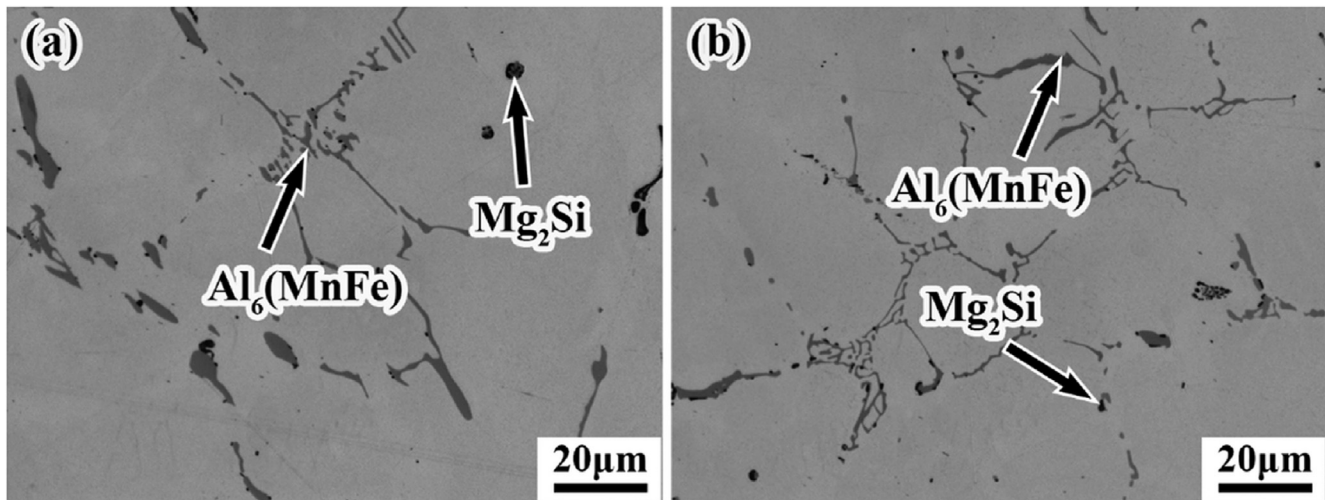
Fig. 1 – As-cast microstructures of (a) B alloy and (b) M alloy.
