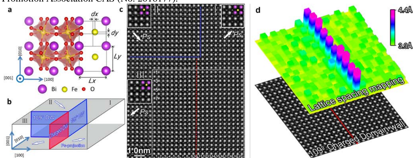
Figure 1. Illustration of 109° CDW of (100) type. (a) Atomic model of multiferroic BFO projected along [001] direction where Bi, Fe and O are represented by violet, yellow, and red spheres, respectively. dx and dy are components of sub-lattice displacement vectors of Fe sub-lattice D_F (from Bi sub-lattice center to Fe sub-lattice) in horizontal and vertical directions. L_x and L_y are the lattice spacing in horizontal and vertical directions. (b) Illustration of intersection of three domains I, II and III, the white arrows are the P_s projections of the corresponding domains along [001] direction. The blue planes are 109° UCDWs of (100) type. The red plane is 109° CDW of (100) type. (c) A HAADF image of domain intersection projected along [001]. The 109° UCDWs of (100) type is marked by blue dotted lines. A red dotted line indicates the 109° CDW of (100) type. The insets are the enlarged images of the corresponding area (violet: Bi, yellow: Fe). The white arrows are the P_s projections. The square frame is the area used for analyzing the lattice variations and Fe sub-lattice displacements. (d) Atomic-level 1D modulation is demonstrated at the negatively charged domain walls in BiFeO 3 thin films. All the 109°, 180°, and 71° charged domain walls of (100) type reveal similar 1D modulations in terms of alternate lattice expansions and clockwise/counterclockwise lattice rotations [6].
